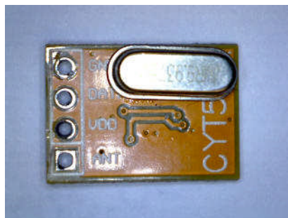
Transmit Module PCB Rear
