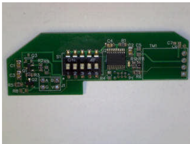
Transmit PCB Front
