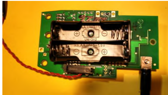
Main PCB Front
