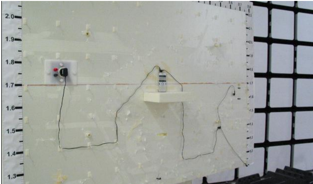
Picture 2. FCC Part 15B Radiated emissions
