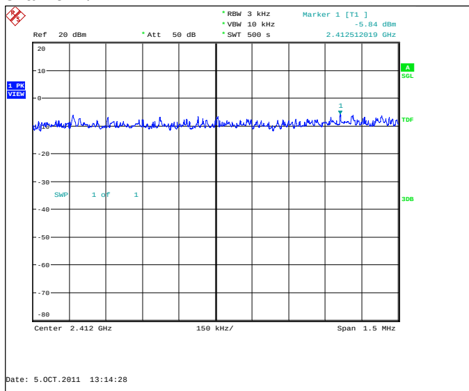
Channel 1 / 2412 MHz
