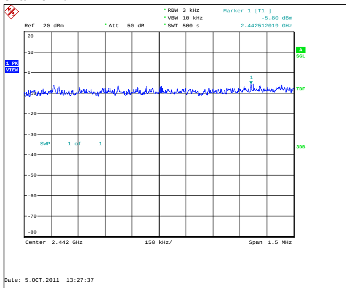
Channel 7 / 2442 MHz
