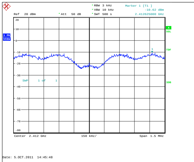
Channel 1 / 2412 MHz
