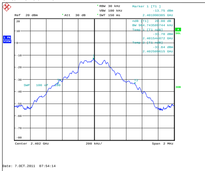
Channel 0 / 2402 MHz
