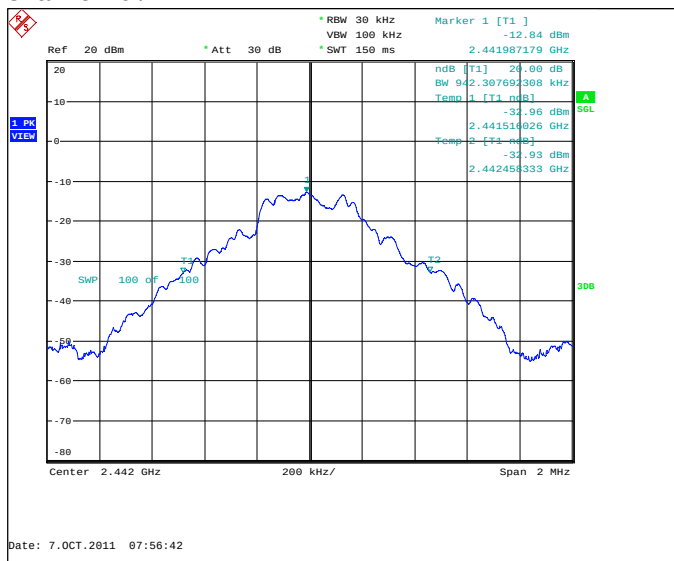
Channel 40 / 2442 MHz
