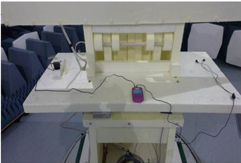
Picture 2. FCC Part 15B Radiated emissions
