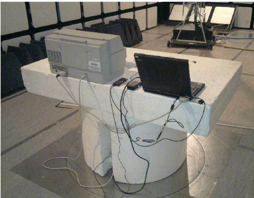
Picture 2. FCC Part 15B Radiated emissions
