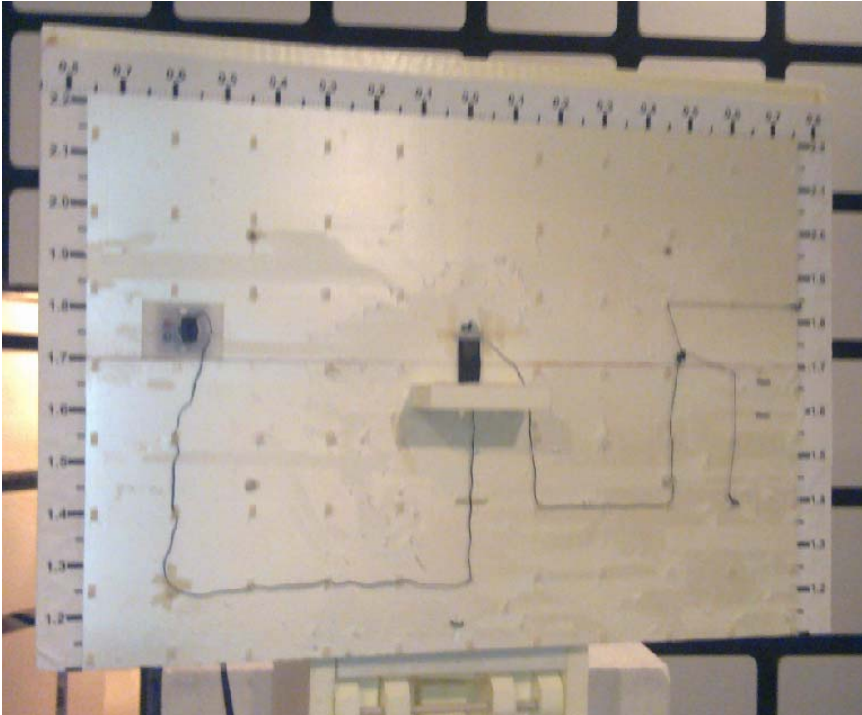
Picture 2. FCC Part 15B Radiated emissions
