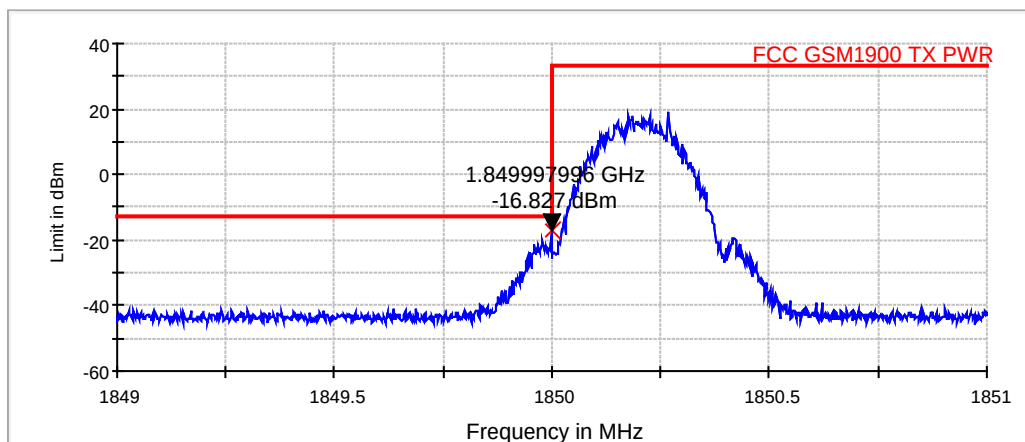
GSM, channel 512 / 1850.2 MHz (Peak detector, RBW: 3 kHz)
