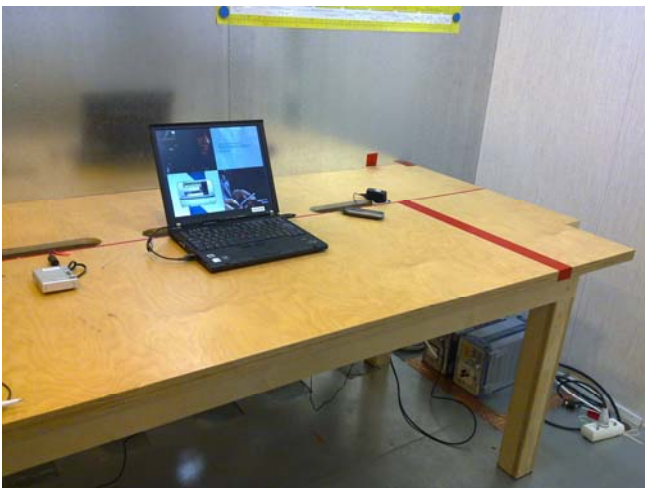
Picture 4 AC powerline conducted emission measurement 15B
