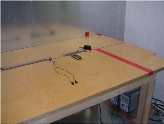
Picture 3 AC powerline conducted emission measurement
