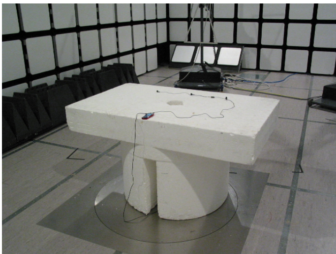
Picture 3 Radiated emission measurement GSM RX + MP3 player on
