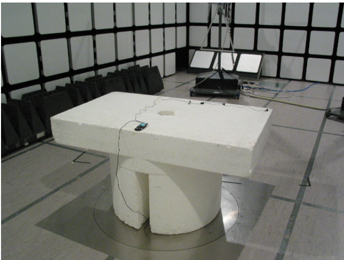
Picture 2 Radiated emission measurement GSM RX / MP3 player on
