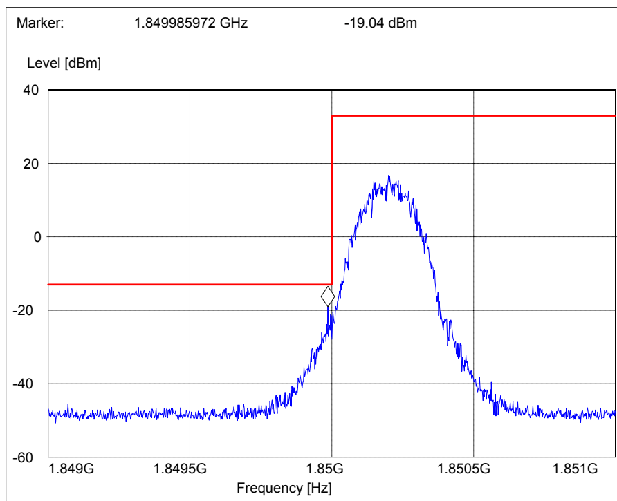
Picture 5 Lower bandedge, channel 512, EGPRS
