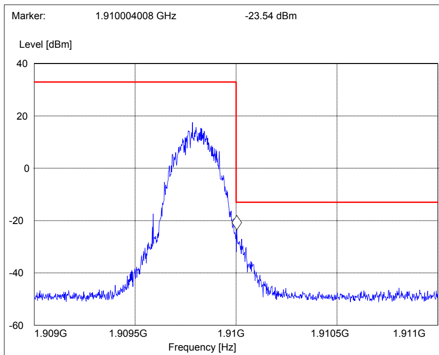
Picture 6 Upper bandedge, channel 810, EGPRS
