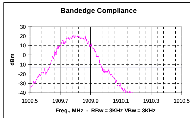
Picture 7. Upper bandedge, channel 810 GSM
