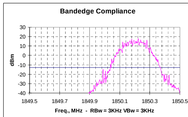
Picture 8. Lower bandedge, channel 512 EGPRS
