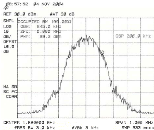
Picture 5. 99% occupied bandwidth, channel 661 EGPRS1900 3KHz Bw and VBw
