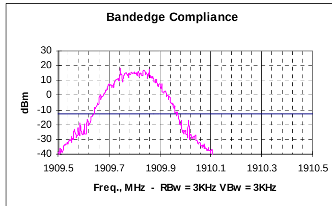
Picture 9. Upper bandedge, channel 810 EGPRS
