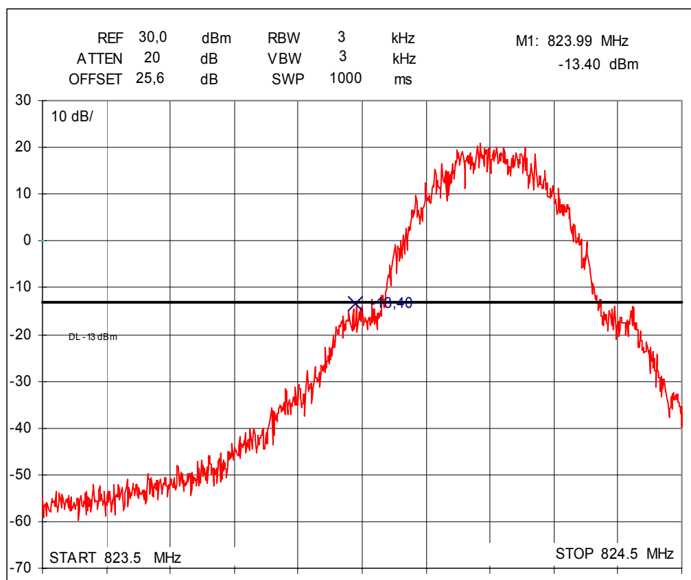
Spectrum analyzer plot channel 128, GMSK modulation
