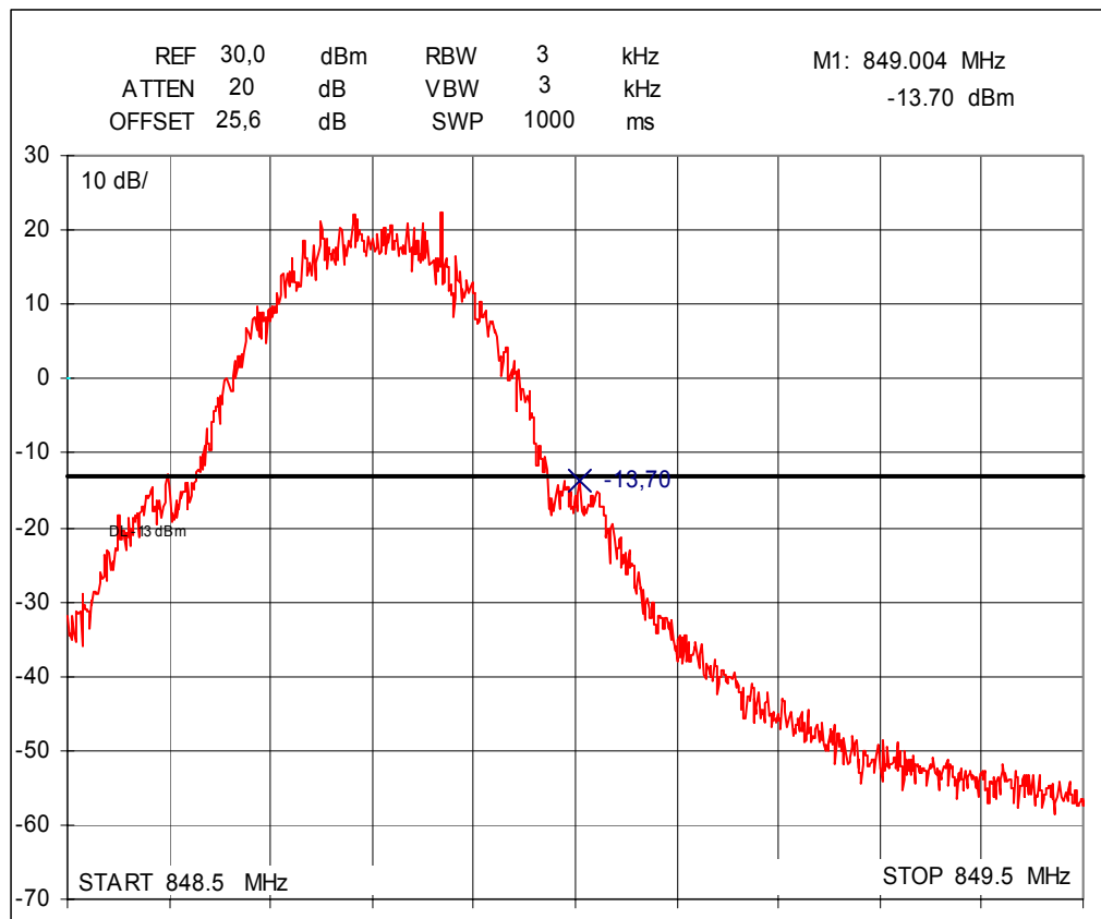
Spectrum analyzer plot channel 251, GMSK modulation
