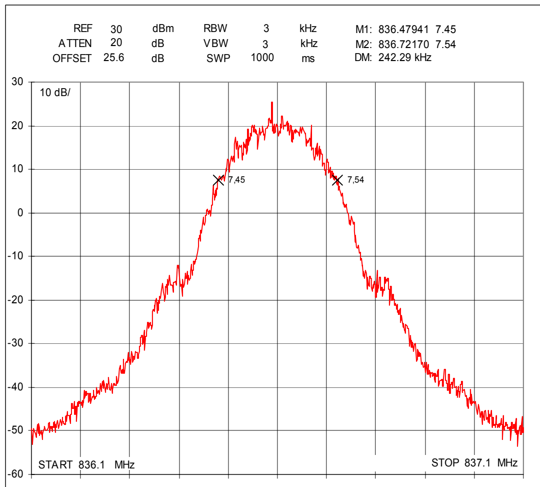
Spectrum analyzer plot channel 190, GMSK modulation
