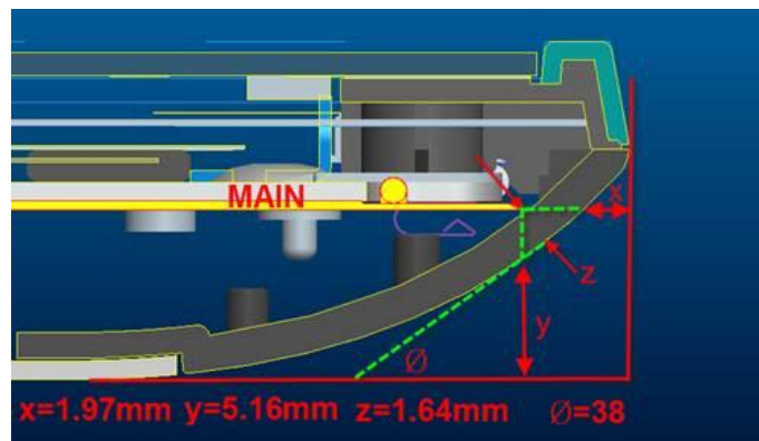
Curved surface of Edge1, Test Separation 0 cm
