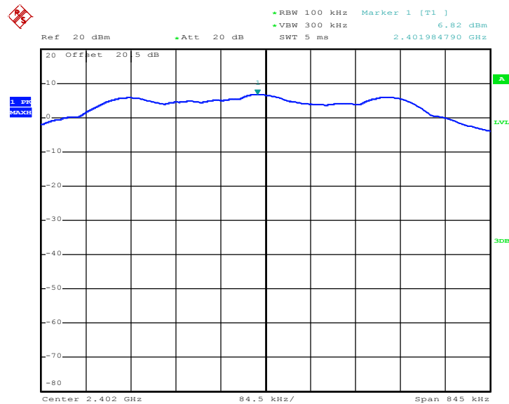
Bluetooth LE PSD Plot on Channel 00
