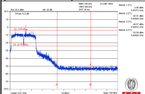
802.11n (40MHz) OFDM MODULATION (CH 110: 5550MHz)
