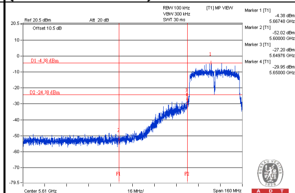
802.11n (40MHz) OFDM MODULATION (CH 134: 5670MHz)
