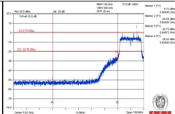
802.11n (20MHz) OFDM MODULATION (CH 132: 5660MHz)
