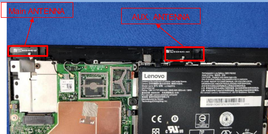
EUT UNCOVER VIEW 2
