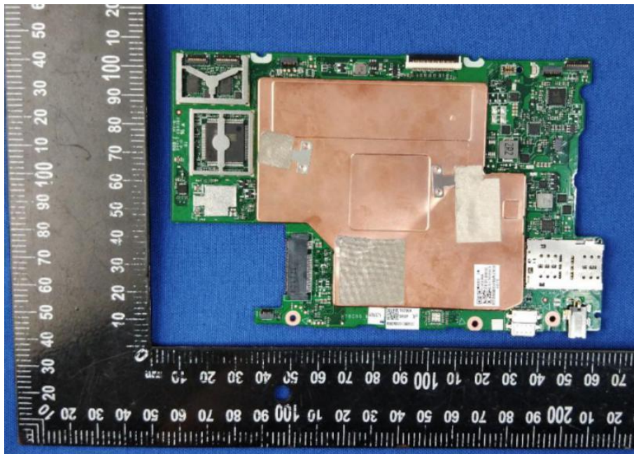
QCNFA425 TOP VIEW (WITH SHIELDING)
