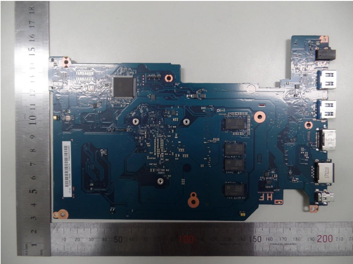
- Mainboard- rear
