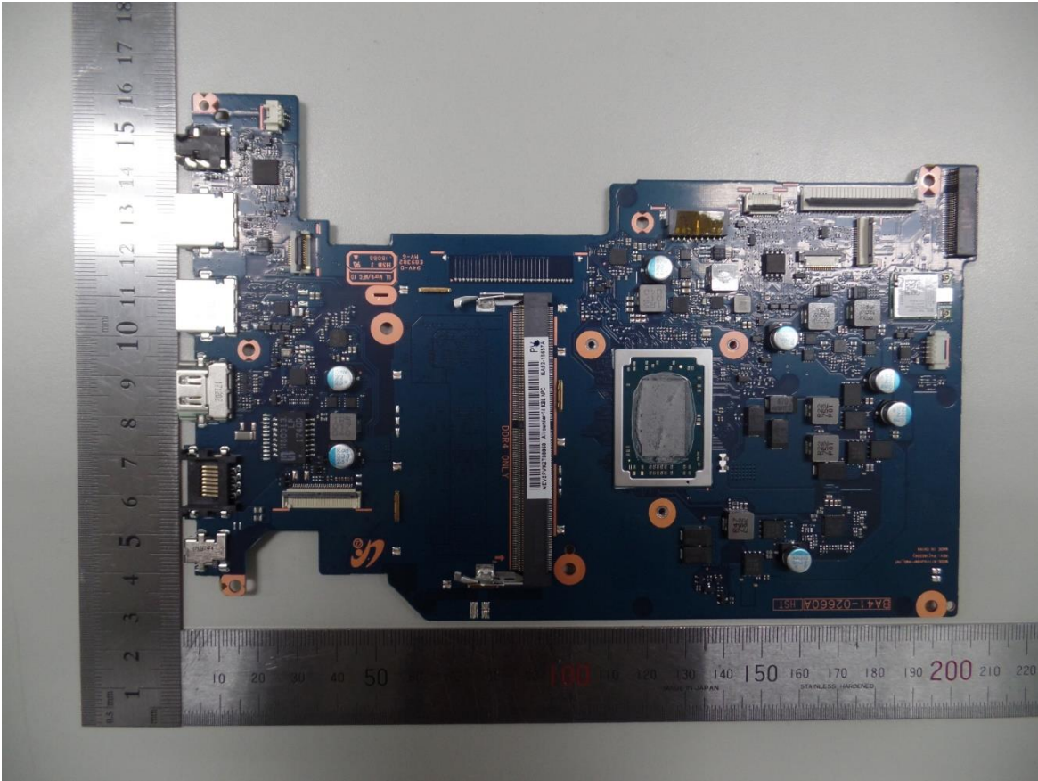
- Mainboard- rear
