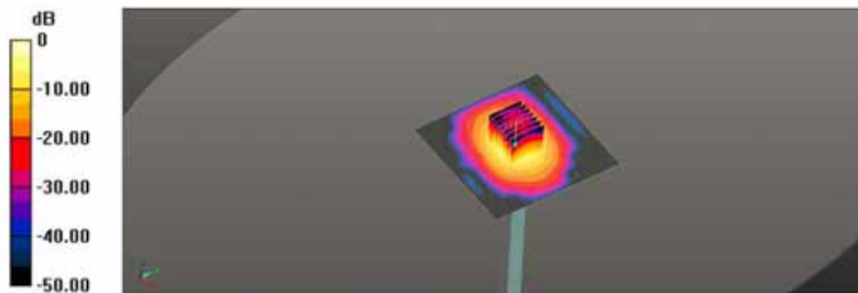
0 dB = 14.2 W/kg = 11.52 dBW/kg
