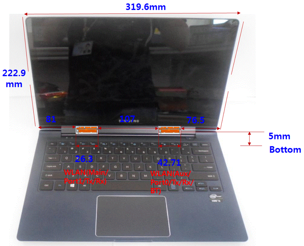
<The Distance information of Antenna to Edges of EUT>
