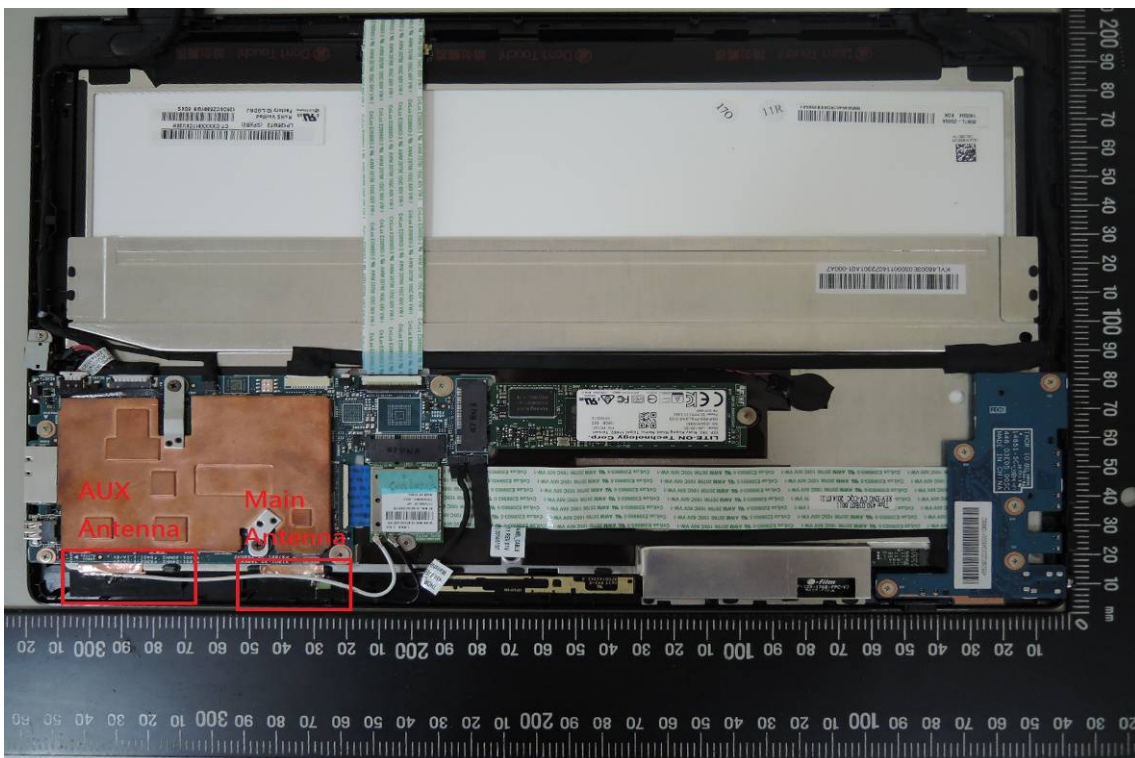
BT/WLAN Antenna Location
