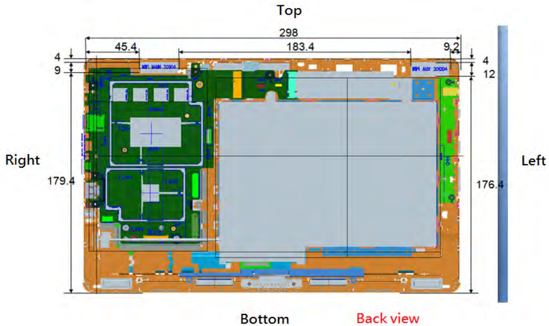
Fig.9 Antenna position of EUT (Back view)
