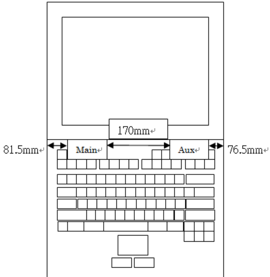
Fig.8 Antenna position of EUT (Front view)
