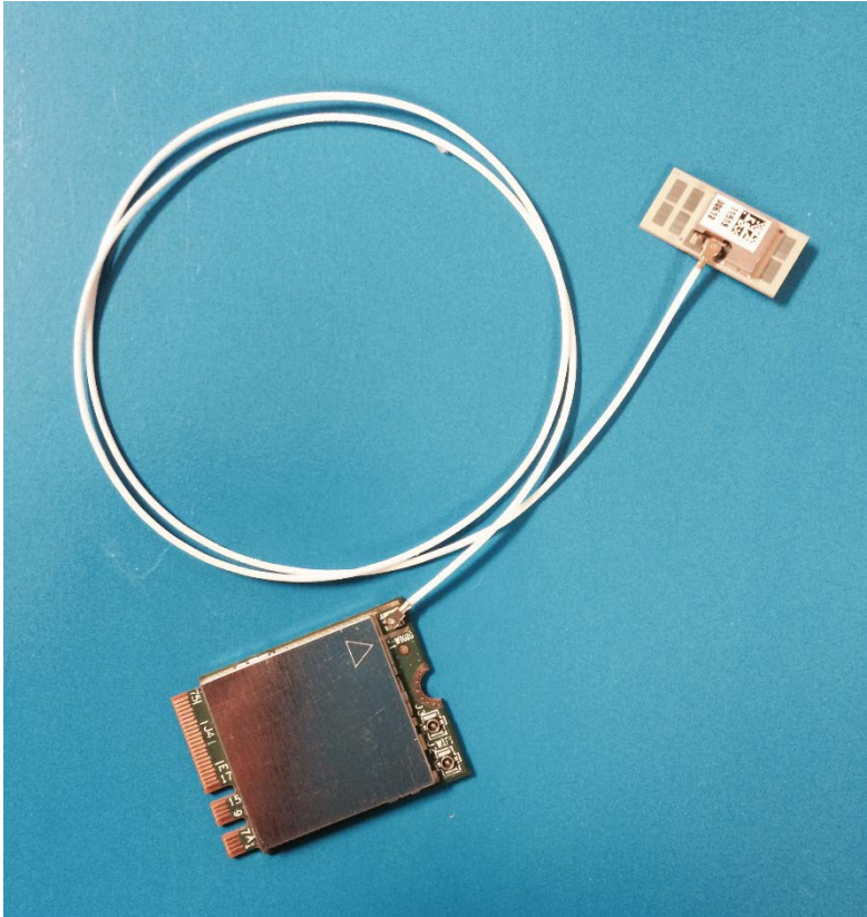
Top View (Entire QCA9008-TBD1 module EUT photo)
