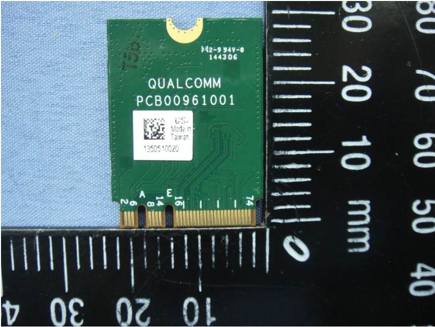
Top View (Entire QCA9008-TBD1 module EUT photo)
