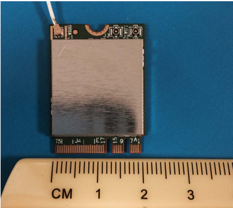
FRONT VIEW (W0096 WiGig BB/WLAN/BT M.2 2230 board)
