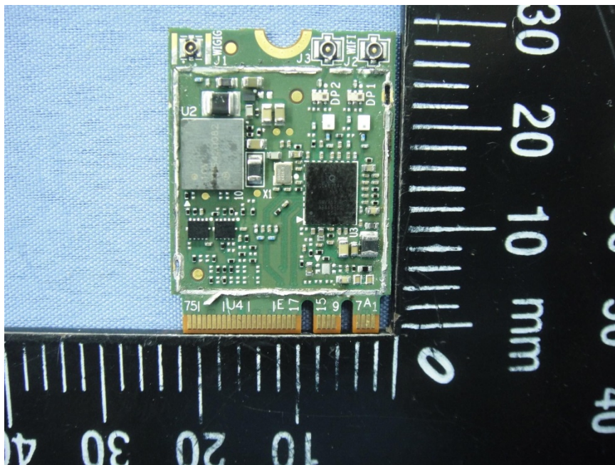
INTERNAL FRONT VIEW (W0096 WiGig BB/WLAN/BT M.2 2230 board)
