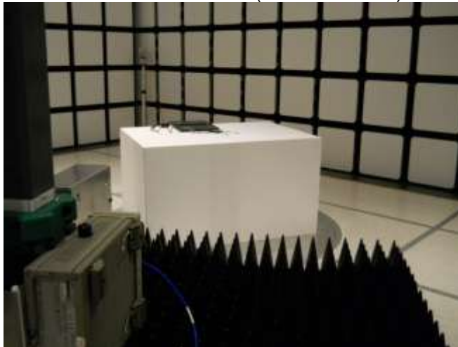
RADIATED BACK PHOTO (ABOVE 1 GHz)
