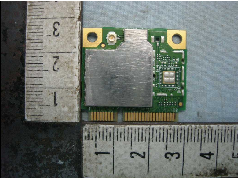
Model: ARS63-D
