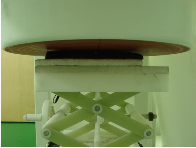
bottom face of tablet PC with Phantom 0 cm Gap
