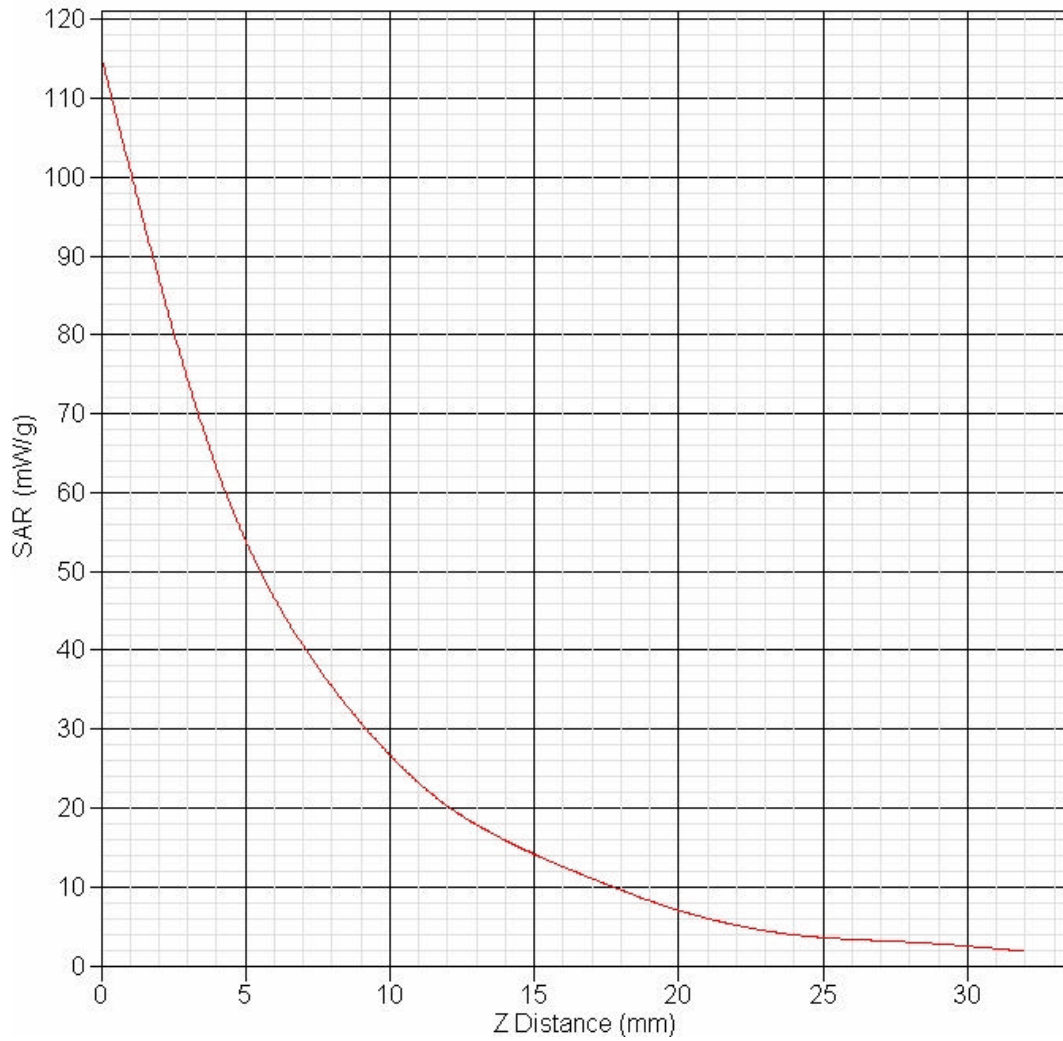
SAR-Z Axis at Hotspot x:0.00 y:0.00
