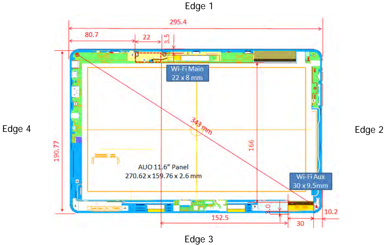
Fig.3 Antenna position of EUT
