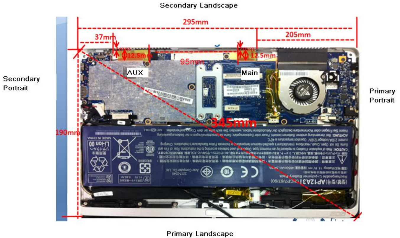
Fig.3 Antenna position of EUT
