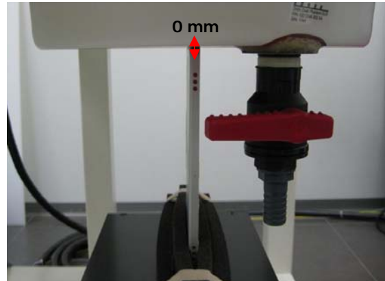
Fig.4 EUT Secondary Portrait mode to flat phantom
