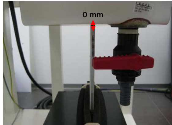
Fig.5 EUT Secondary Landscape mode to flat phantom
