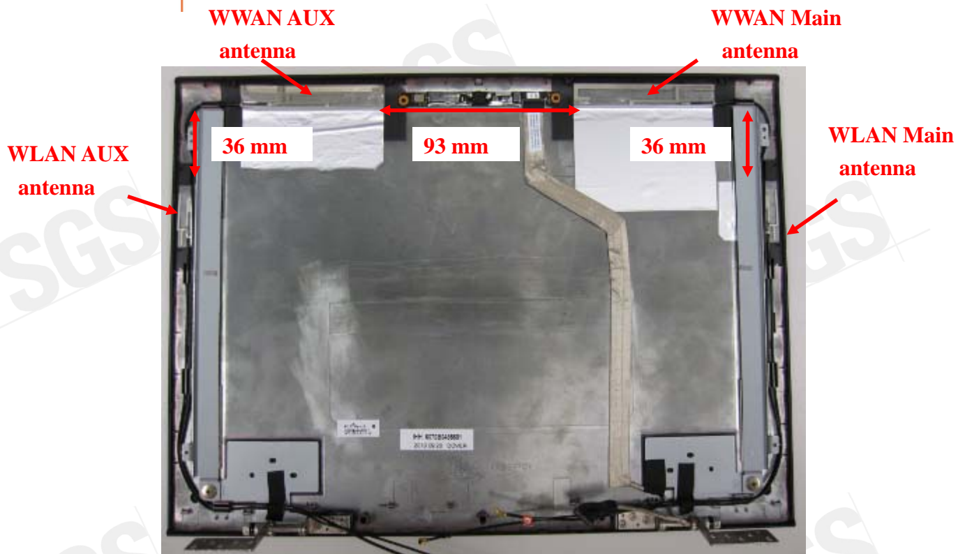
Antenna position of EUT
