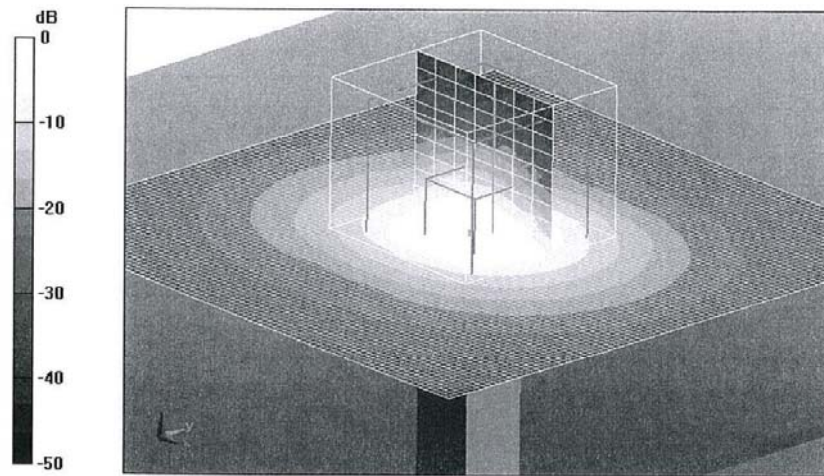
0 dB = 15mW/g
