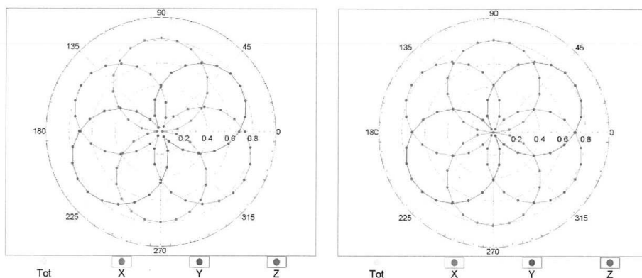
f=600 MHz,TEM
