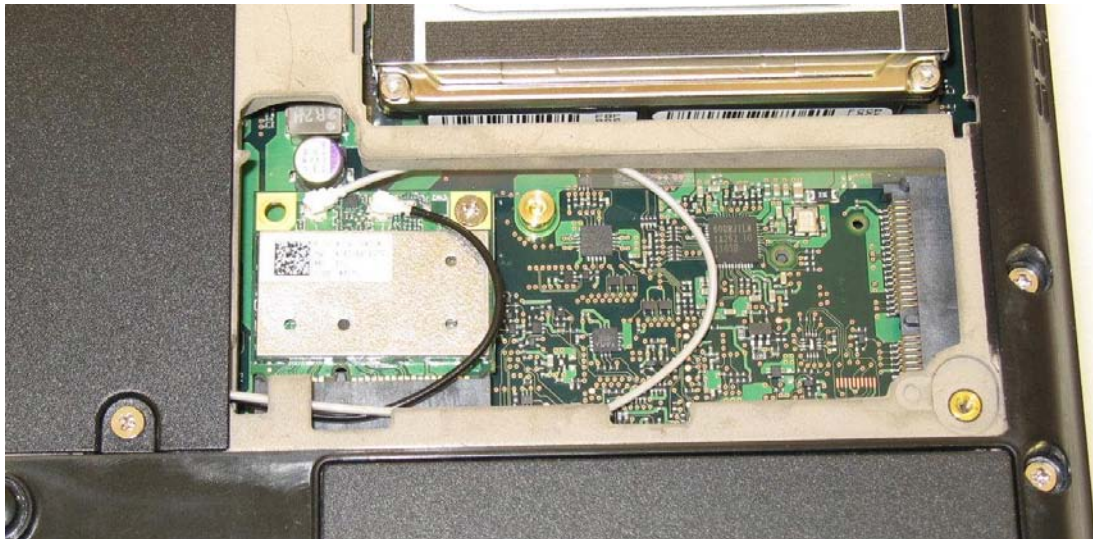
AR5BHB116 inside the Fujitsu TABLET Computer
