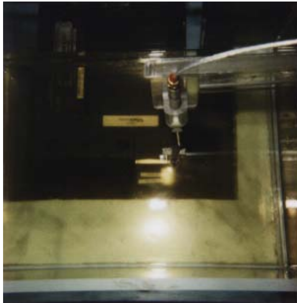
Fig. 3. Photograph of the Atheros Model AR5BCB-00022 CardBus Card inserted into a laptop computer with its bottom pressed against the bottom of the planar tissue-simulant phantom to simulate "above-lap" placement of the wireless PC. A Styrofoam block is used under the base to prevent bending of the 2 mm thin base of the phantom.
