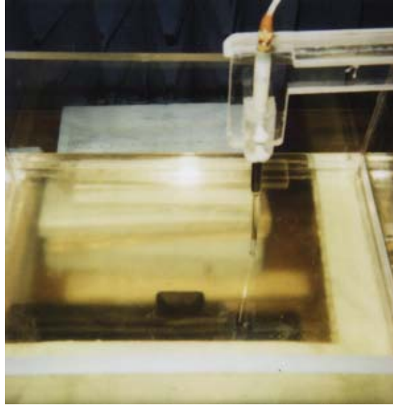
Fig. 4. Photograph of the Atheros Model AR5BCB-00022 CardBus Card inserted into a portable computer (as in Fig. 1) placed with the card edge at 90° and separated from the bottom of the phantom by 2.5 cm for "end-on" testing of SAR. As in Fig. 3, here too, a Styrofoam block is used under the base to prevent bending of the 2 mm thin base of the phantom.
