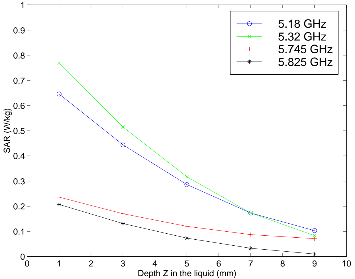
Fig. 5. Plot of the SAR variations as a function of depth Z in the liquid for locations of highest SAR (from Tables 1-4 -- Above-lap position) for Atheros Model AR5BCB-00022 CardBus Card.
