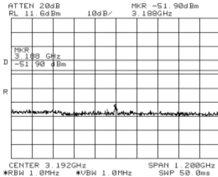
T45059/812 (3 GHz)
