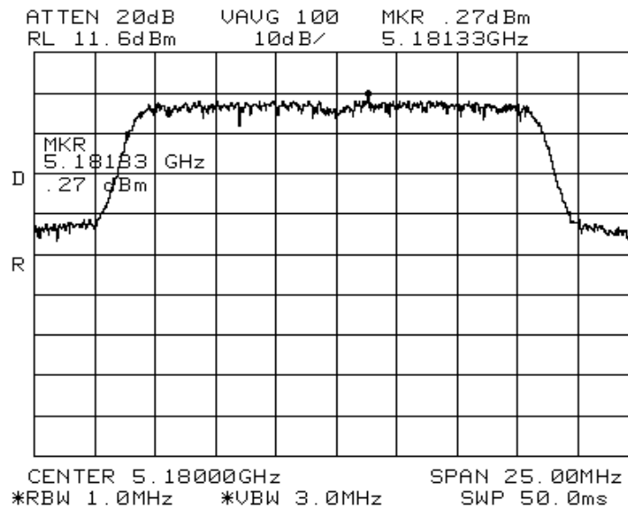
T45059 / 203 @ 13.8 dBm
