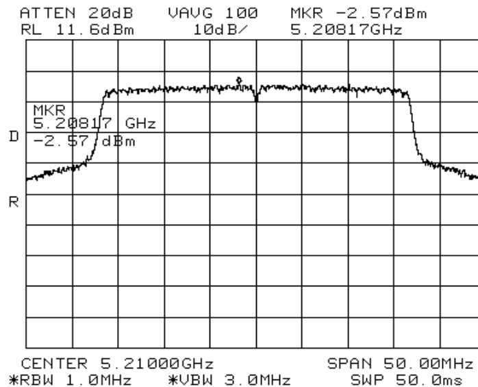
T45059 / 903 @ 13.8 dBm
