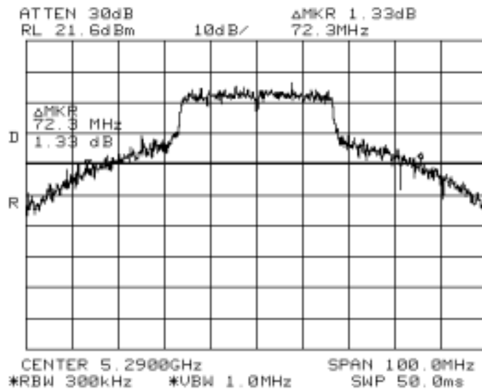
T45059 / 1003 @ 17.5 dBm
