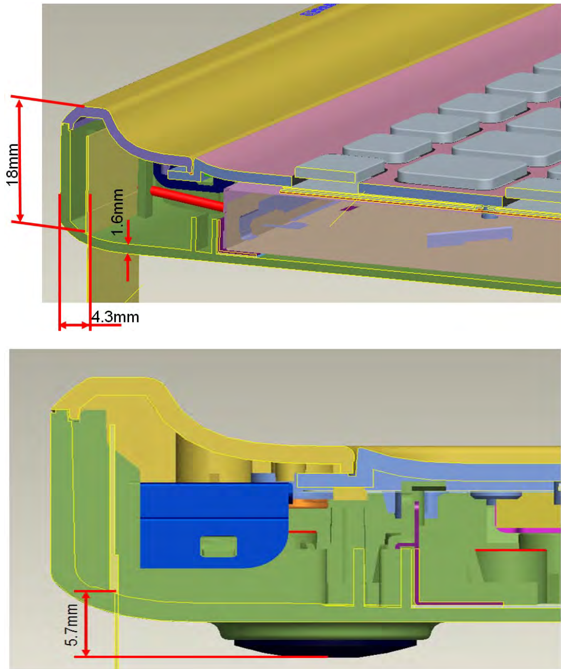
Fig.6 Main Antenna position of EUT
