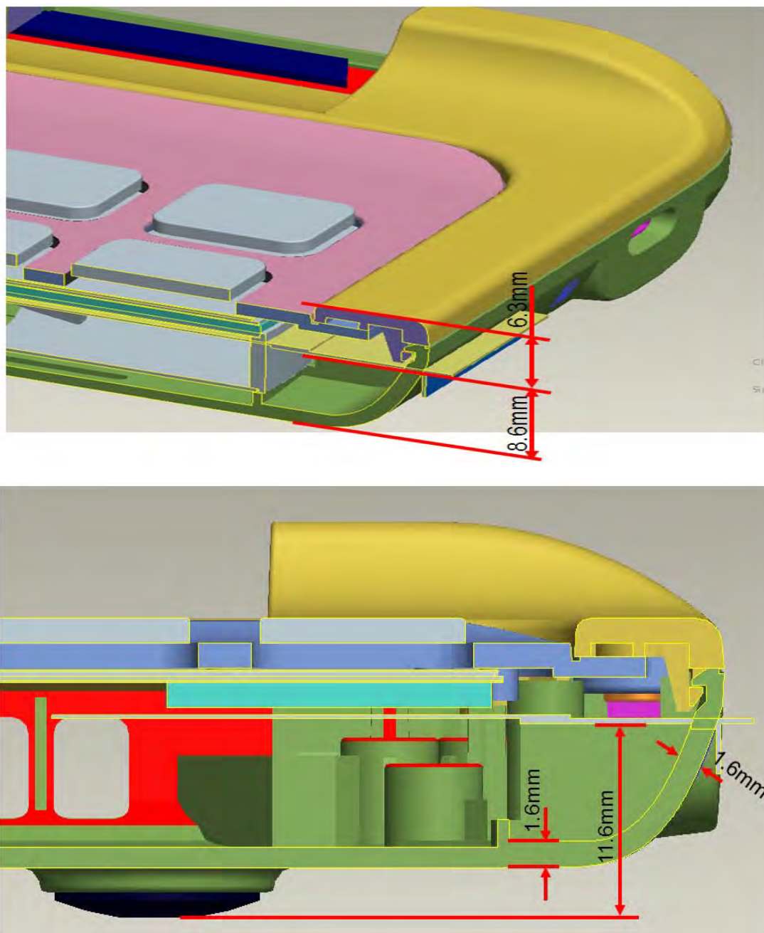
Fig.7 Aux Antenna position of EUT
