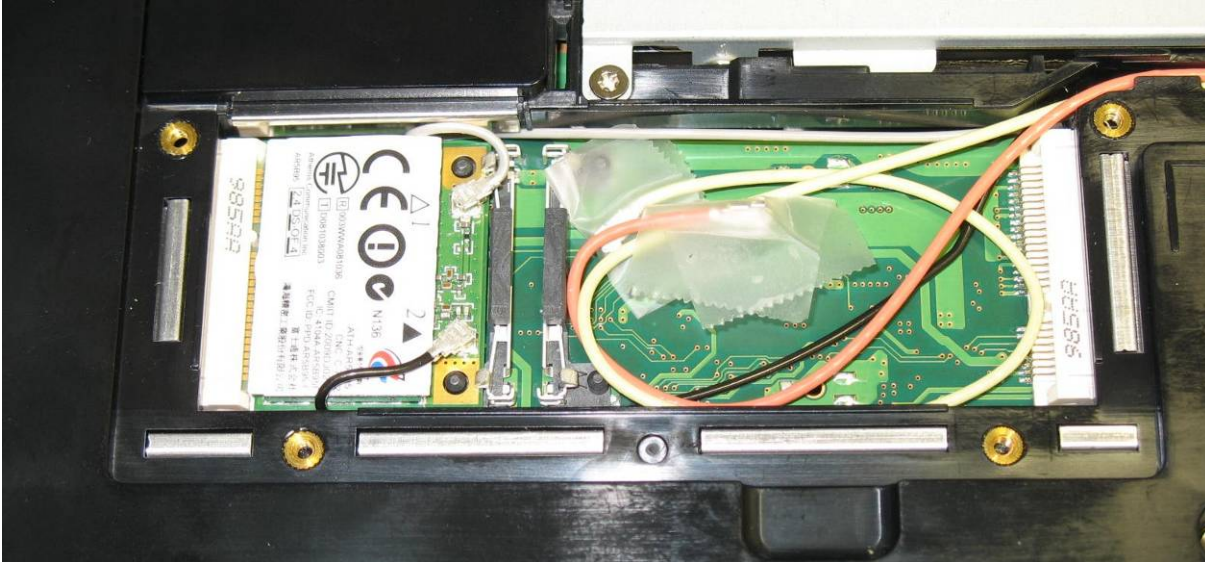
AR5B95 inside the Fujitsu Notebook Computer
