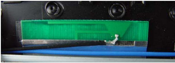
Tx1 Antenna
