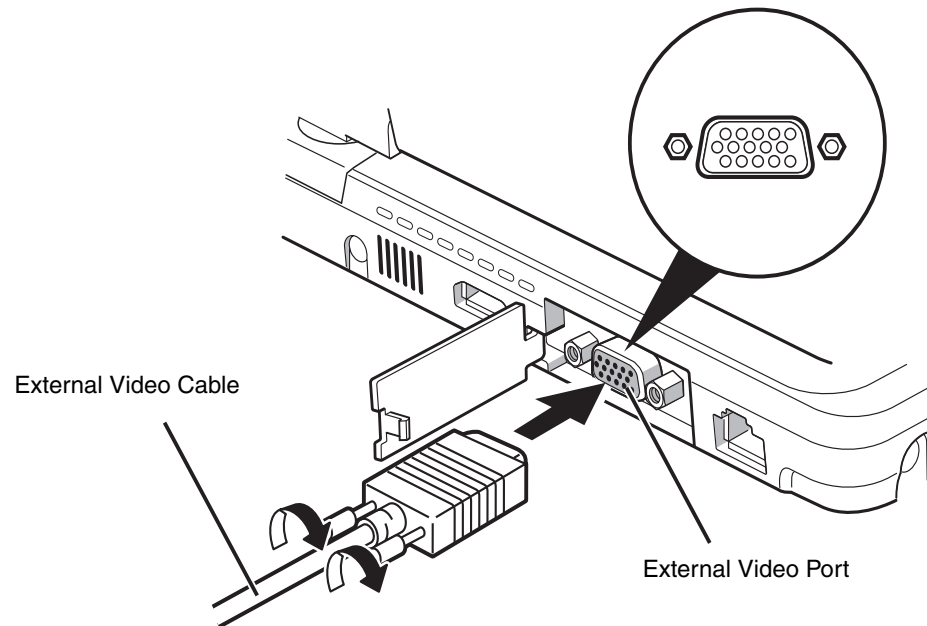
Figure 48. Connecting an External Video Device
