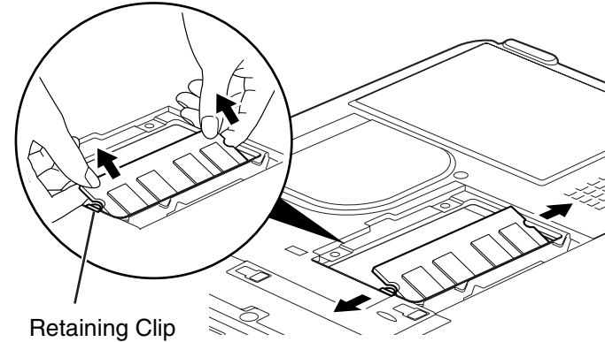
Figure 40. Installing a Second Memory Module
