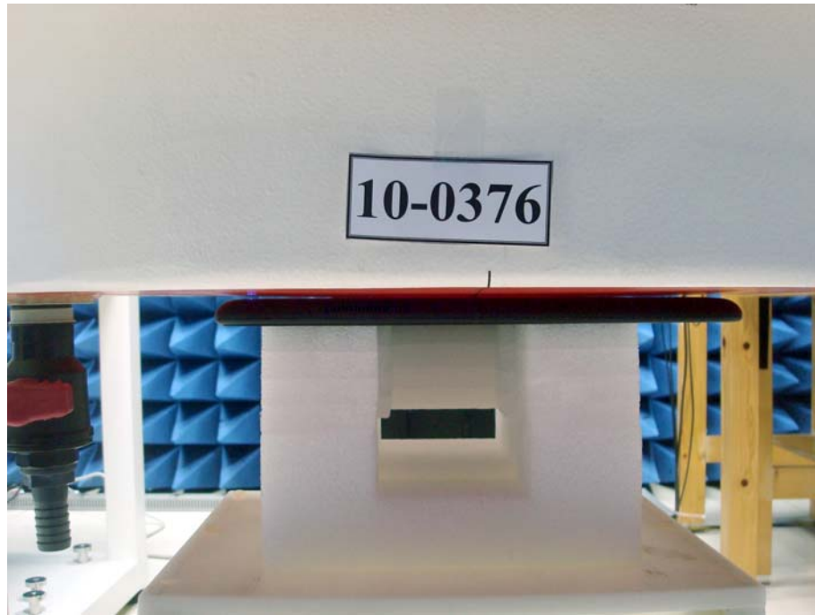
Figure 1. Body SAR Test Setup (Flat Section) Host Bottom Close Body
