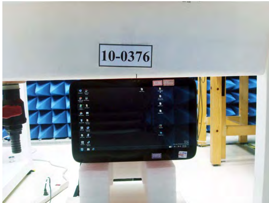
Figure 2. Body SAR Test Setup (Flat Section) Host Secondary Landscape Close Body
