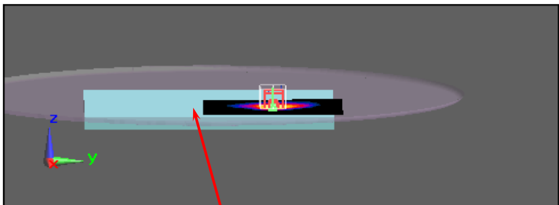
Figure 1. Body SAR Test Setup (Flat Section) Host Bottom Close Body
