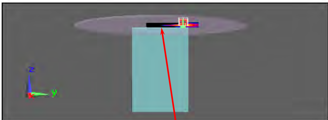
Figure 3. Body SAR Test Setup (Flat Section) Host Primary Portrait Close Body
