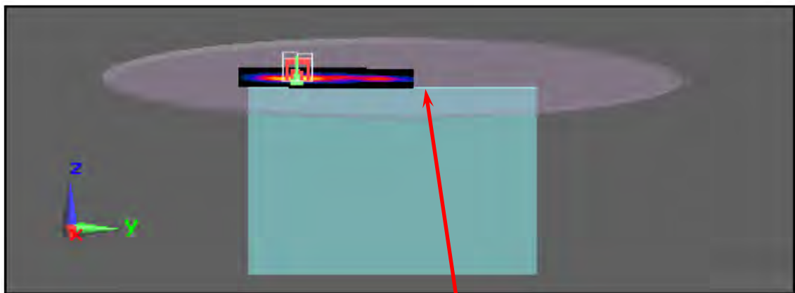
Figure 2. Body SAR Test Setup (Flat Section) Host Secondary Landscape Close Body
