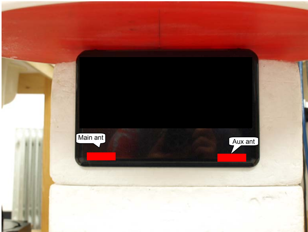
Laptop Mode with Flat Phantom (
