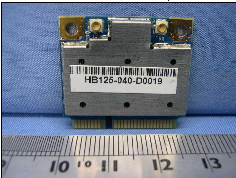
EUT <Version B(Dual antenna)>
