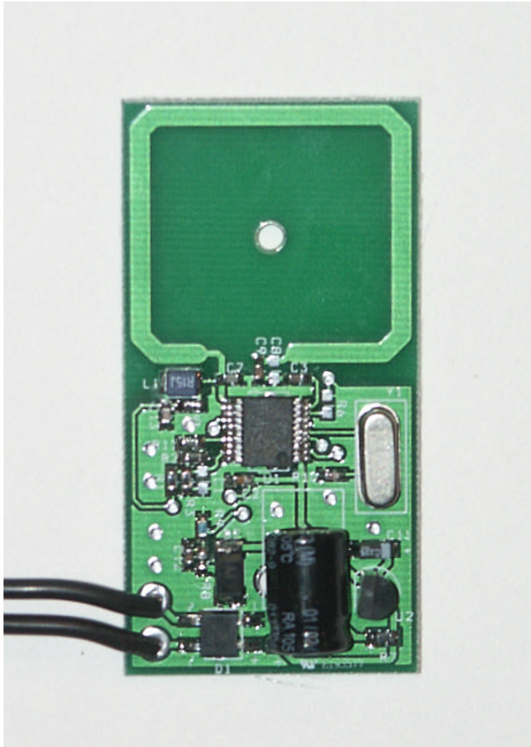
Transmitter Circuit Board Top View
