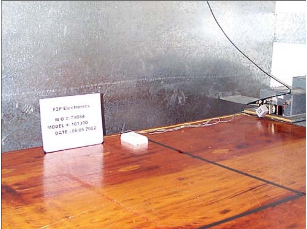
Receiver Conducted Emissions - Front View
