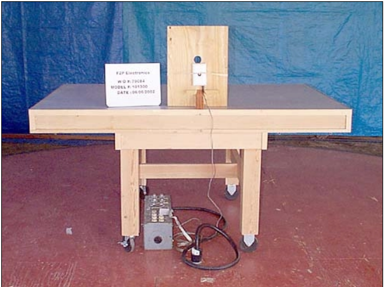
Receiver Radiated Emissions - Front View
