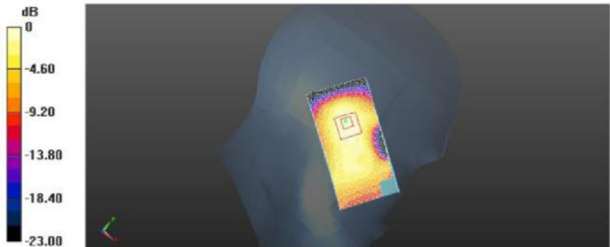
Plot 2: Left Head Tilt (GSM850 Middle Channel)
