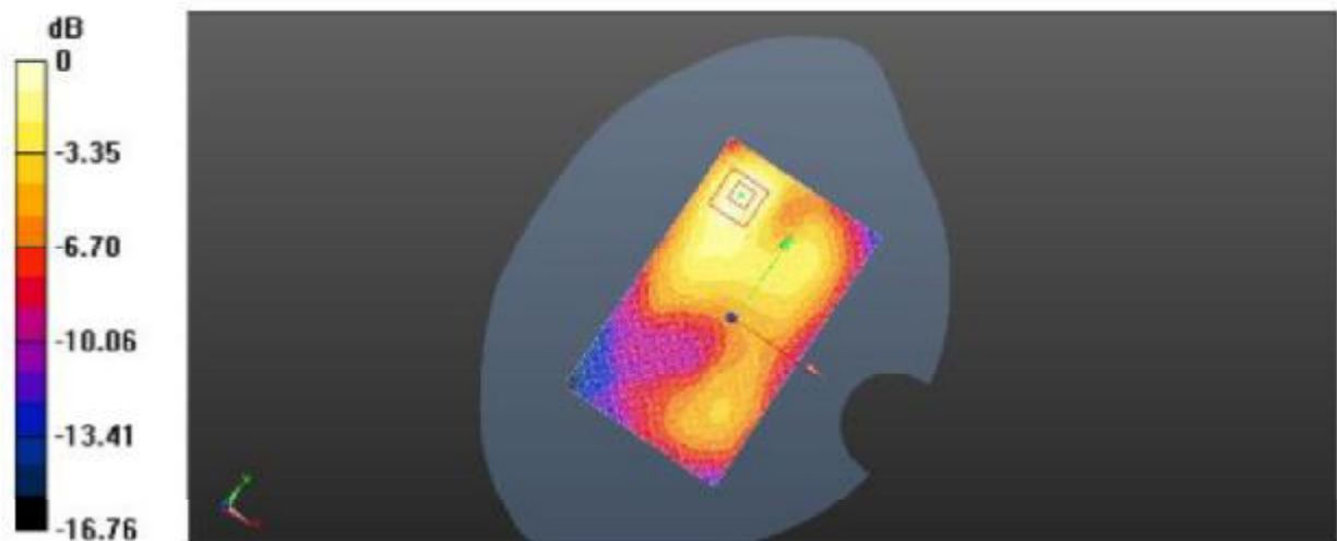
Plot 6: Body Rear Side (GSM850 GPRS 4TS Middle Channel)
