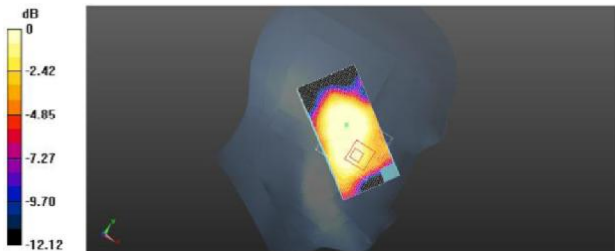
Plot 12: Left Head Tilt (PCS1900 Middle Channel)
