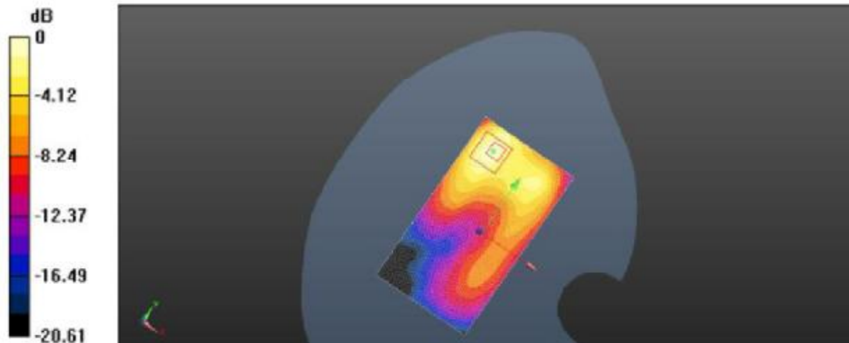
Plot 20: Body Rear Side (PCS1900 Specch With Headset Middle Channel)
