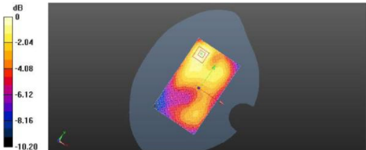
Plot 10: Body Rear Side (GSM850 Speech With Headset Middle Channel)
