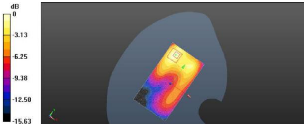
Plot 8: Body Right Side (GSM850 GPRS 4TS Middle Channel)
