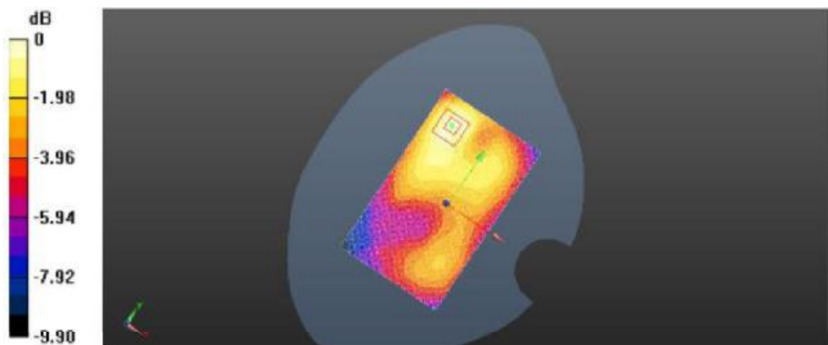
Plot 19: Body Bottom Side (PCS1900 GPRS 4TS Middle Channel)
