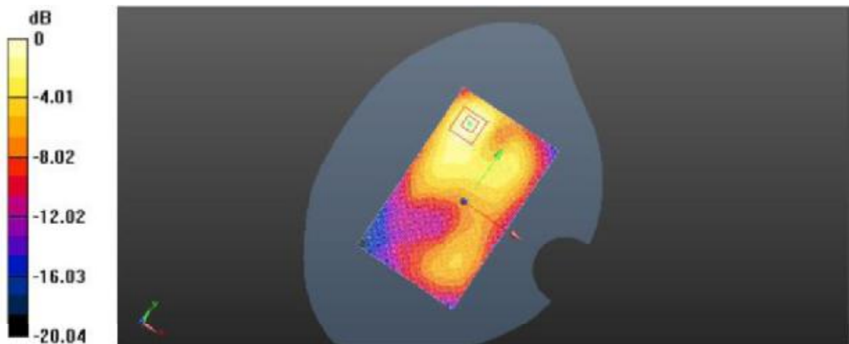
Plot 9: Body Bottom Side (GSM850 GPRS 4TS Middle Channel)
