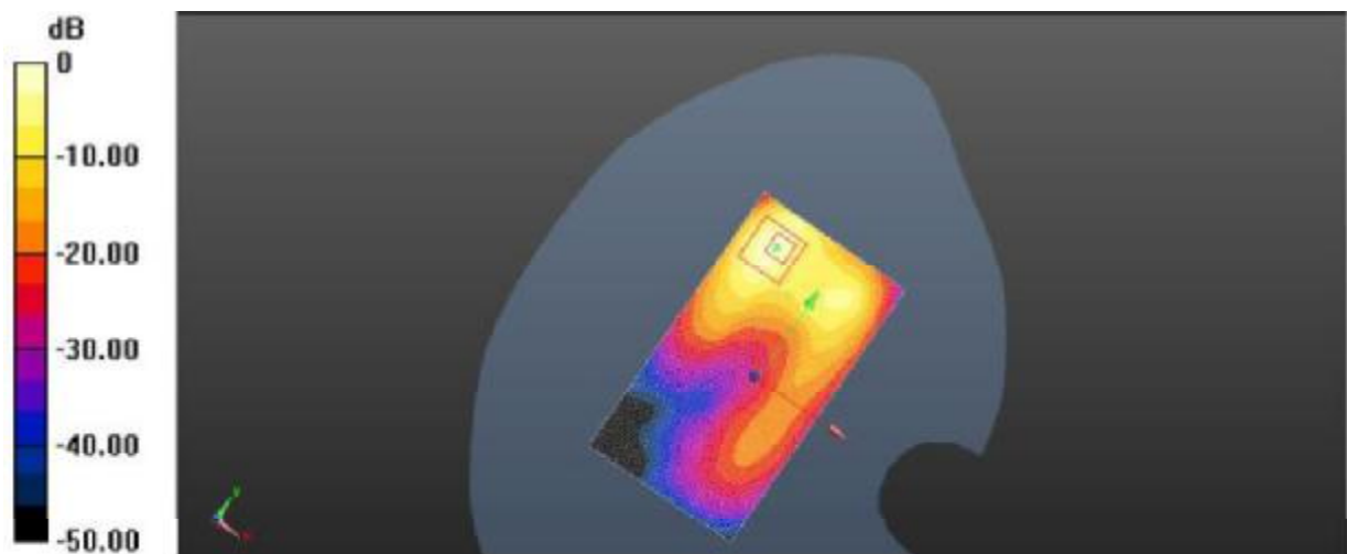
Plot 18: Body Right Side (PCS1900 GPRS 4TS Middle Channel)
