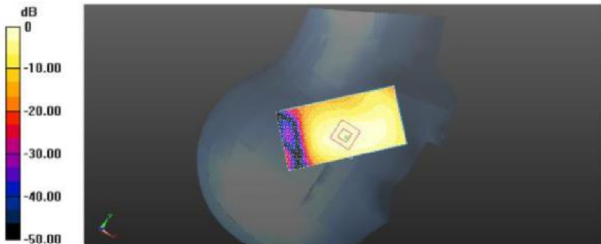
Plot 3: Right Head Touch (GSM850 Middle Channel)
