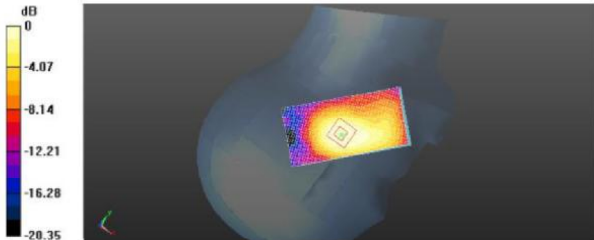
Plot 14: Right Head Tilt (PCS1900 Middle Channel)
