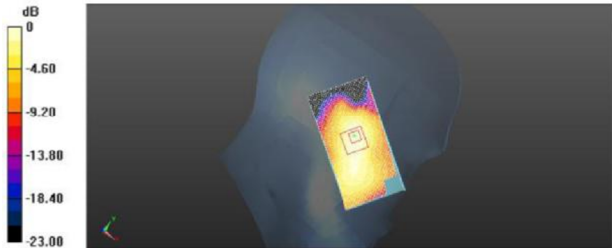
Plot 11: Left Head Touch (PCS1900 Middle Channel)
