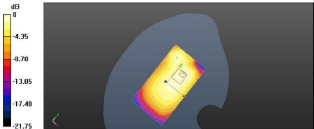
Plot 7: Body Left Side (GSM850 GPRS 4TS Middle Channel)
