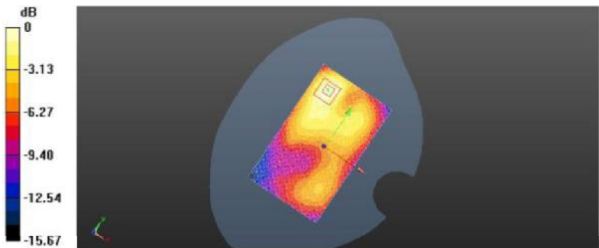
Plot 15: Body Front Side (PCS1900 GPRS 4TS Middle Channel)
