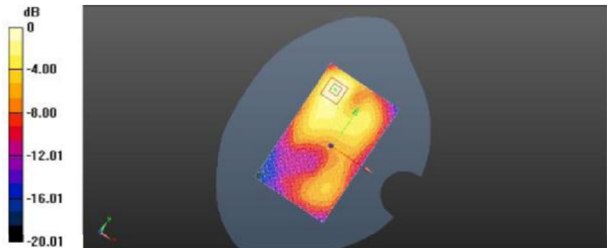
Plot 17: Body Left Side (PCS1900 GPRS 4TS Middle Channel)
