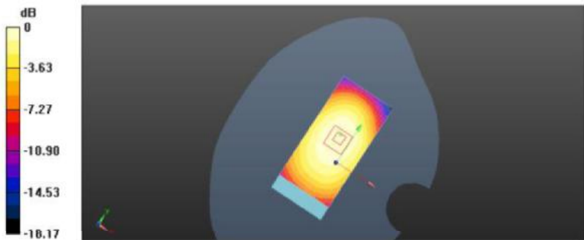
Plot 5: Body Front Side (GSM850 GPRS 4TS Middle Channel)
