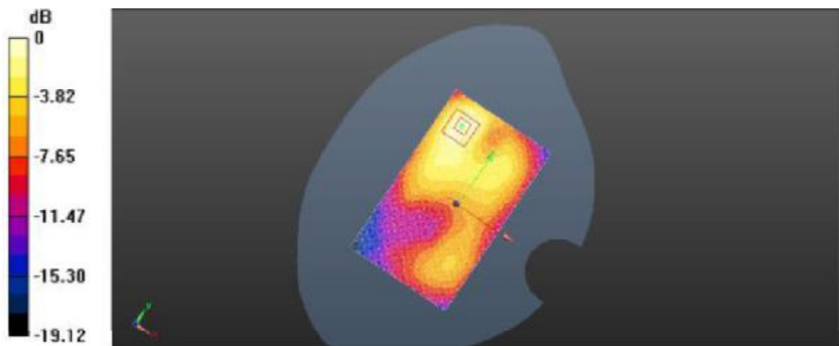
Plot 16: Body Rear Side (PCS1900 GPRS 4TS Middle Channel)
