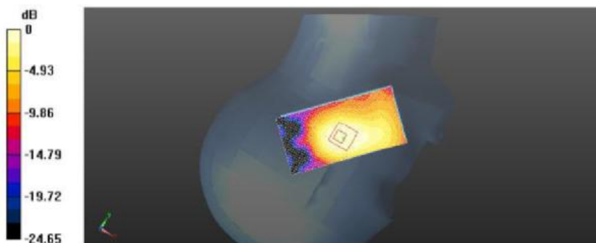
Plot 13: Right Head Touch (PCS1900 Middle Channel)
