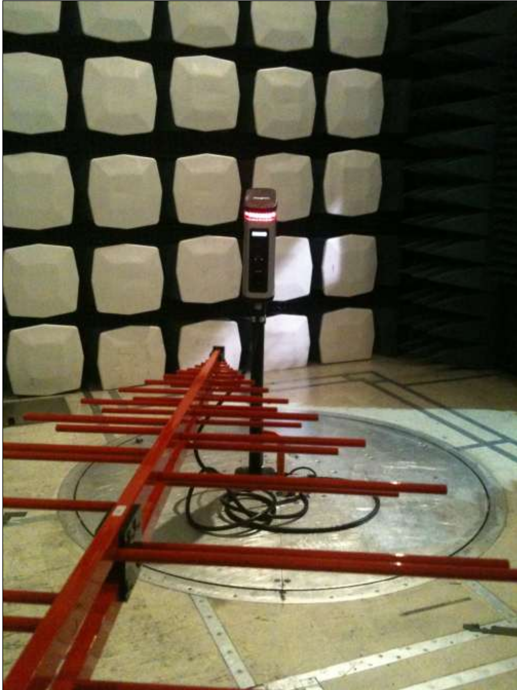
Photograph 6. Radiated Spurious Emissions, Below 1 GHz, Test Setup
